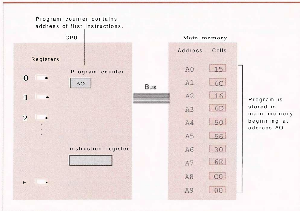
Figure 2.10J The program from Figure 2.7 stored in main memory ready for execution
