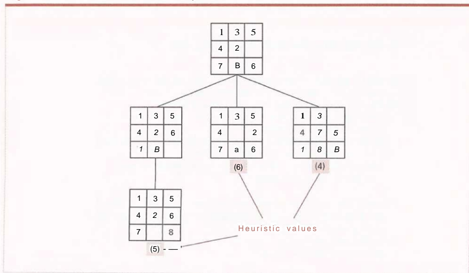
Figure 10.12 The search tree after two passes
