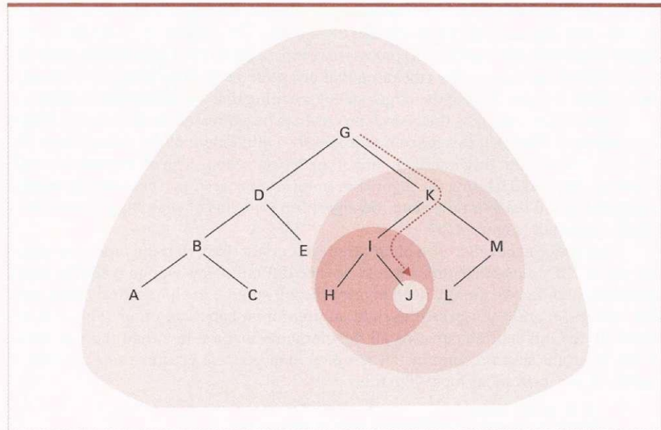
Figure 8.21 The successively smaller trees considered by the procedure in Figure 8.20 when searching for the letter J
