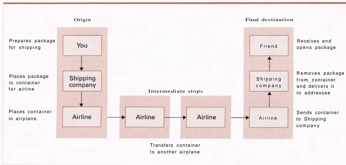
Figure 4.12 Package-shipping example
