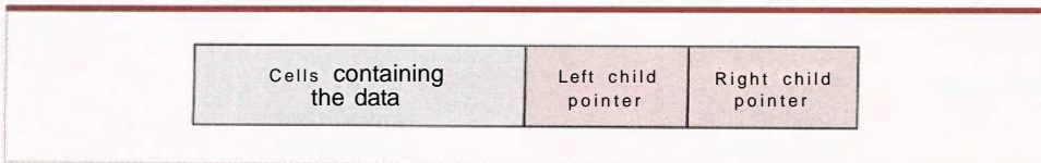
Figure 8.14 The structure of a node in a binary tree
