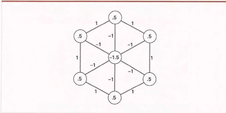
Figure 10.22 An artificial neural network implementing an associative memory
