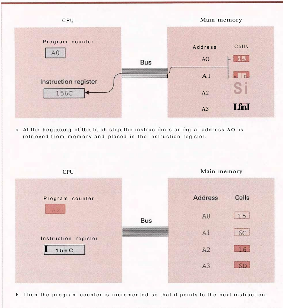
Figure 2.11 Performing the (etch step of the machine cycle
