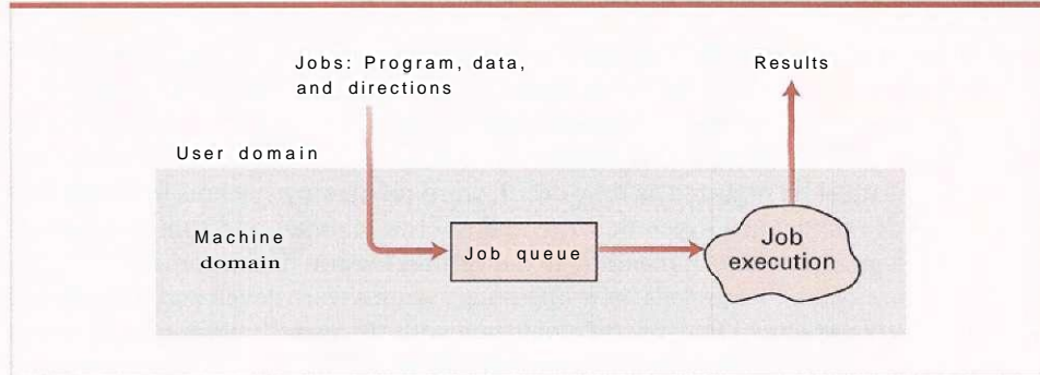
Figure 3.1 Batch processing
