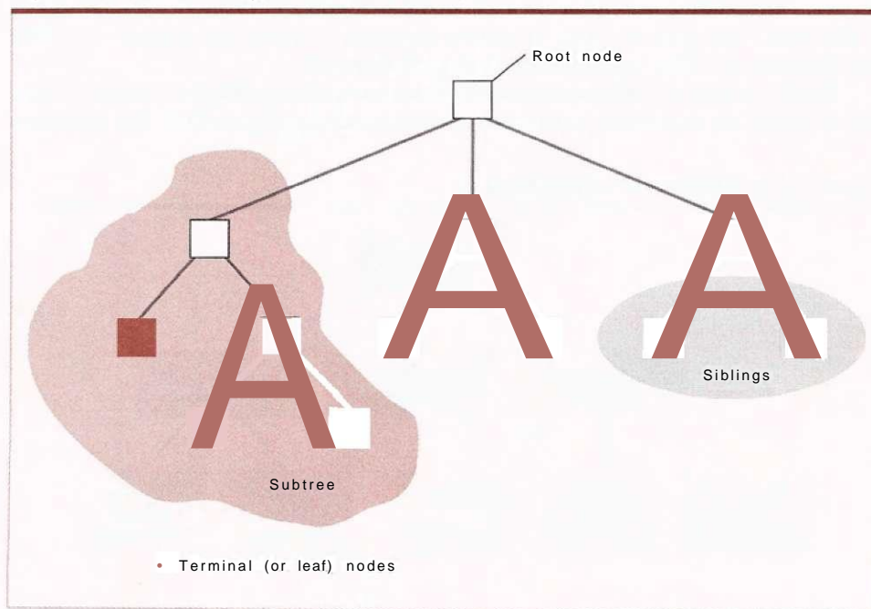
Figure 8.3 Tree terminology
