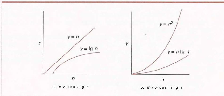
Figure 1).11 Graphs of the mathematical expressions n versus \lg n , and n^2
