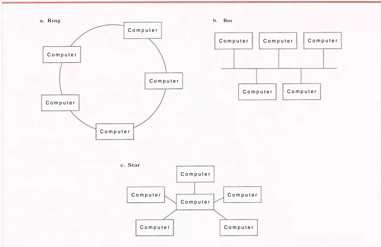
Figure 4.1 Network topologies
