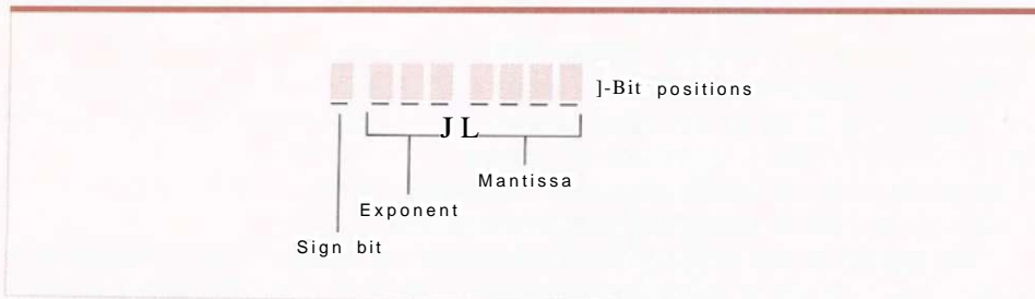
Figure 1.26 Floating-point notation components
