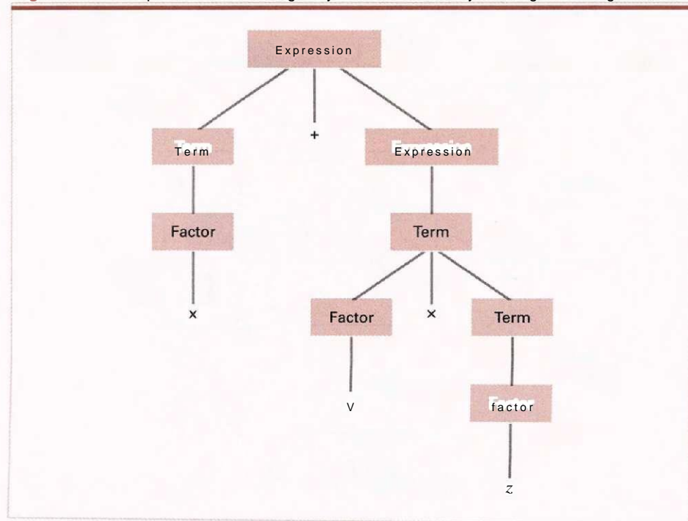
Figure 6.17 The parse tree for the string x + y x z based on the syntax diagrams in Figure 6.16
