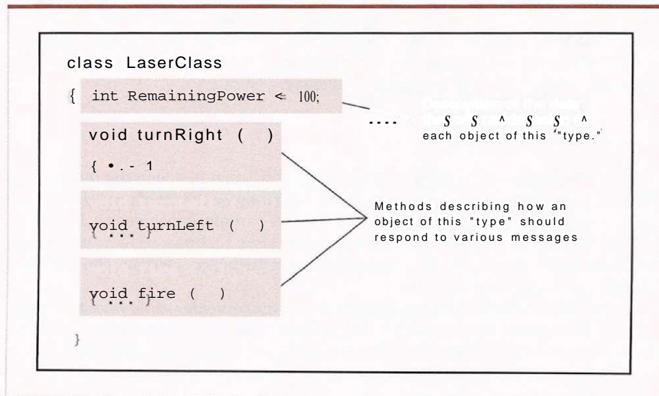
Figure 6.20 The structure of a class describing a laser weapon in a computer game
