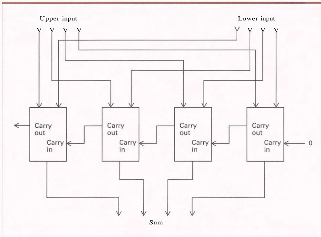
Figure B.3 A circuit for adding two values in a two's complement notation using four copies of the circuit in Figure 8.2
