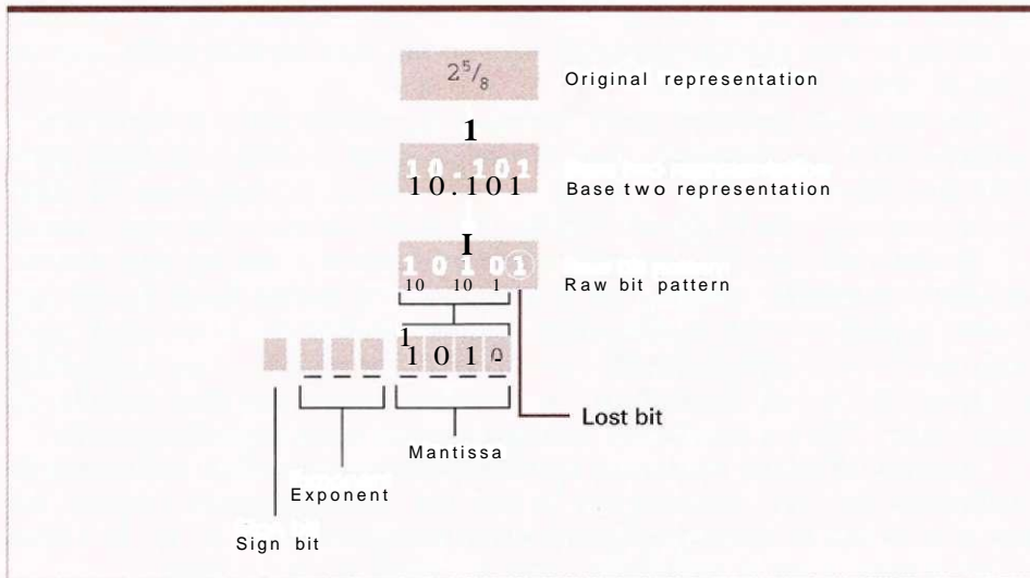
Figure 1.27 Encoding the value 2\%
