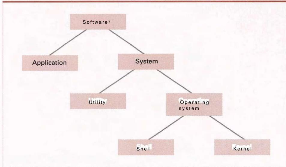
Figure 3.3 Software classification
