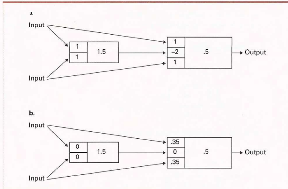
Figure 10.18 A neural network with two different programs
