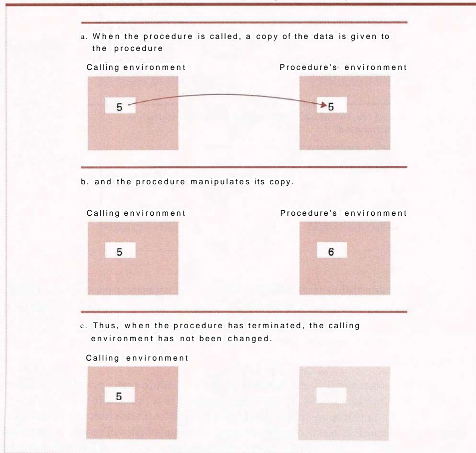
Figure 6.11 Executing the procedure Demo and passing parameters by value
