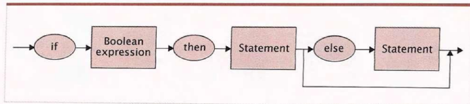
Figure 6.15 A syntax diagram of our if-then-else pseudocode statement
