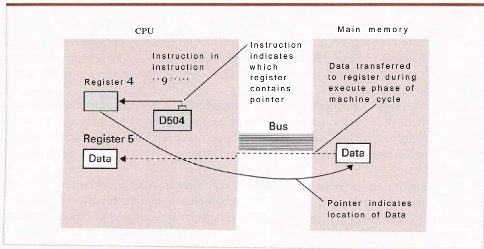
Figure 6.28 Loading a register from a memory cell that is located by means of a pointer stored in a register
