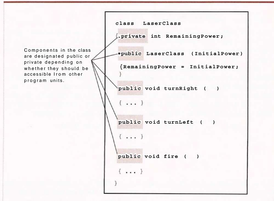
Figure 6.22 Our LaserClass definition using encapsulation as if would appear in a Java or C# program
