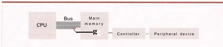
Figure 2.14 A conceptual representation of memory-mapped I/O
