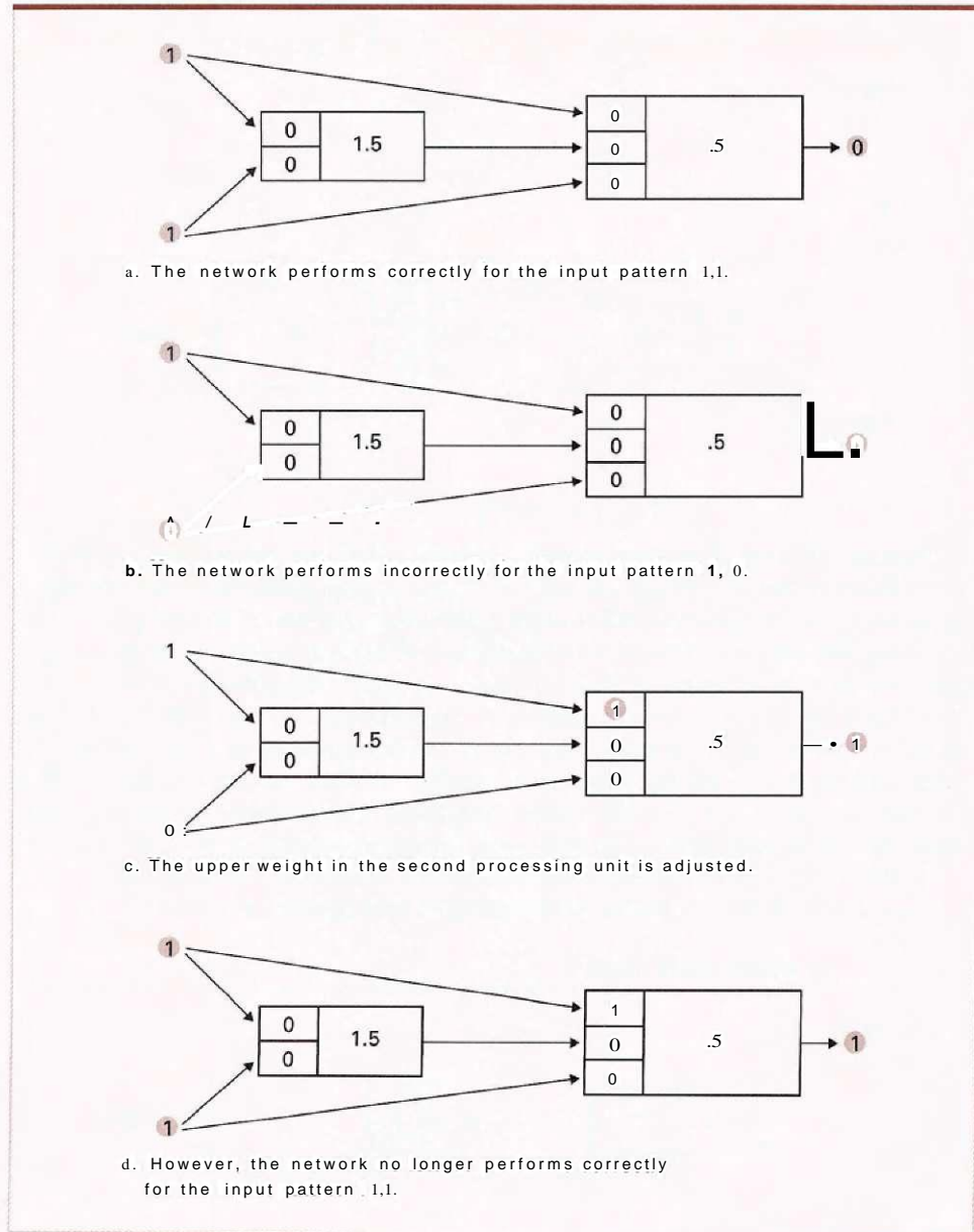
Figure 10.20 Training an artificial neural network
